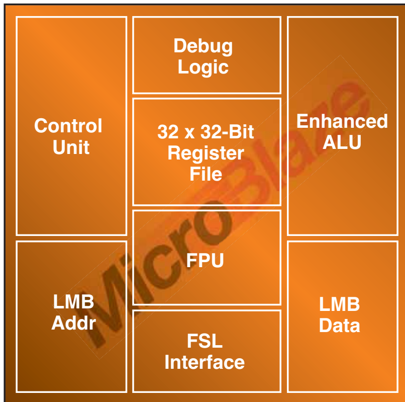
Figure 1 – MicroBlaze block diagram
