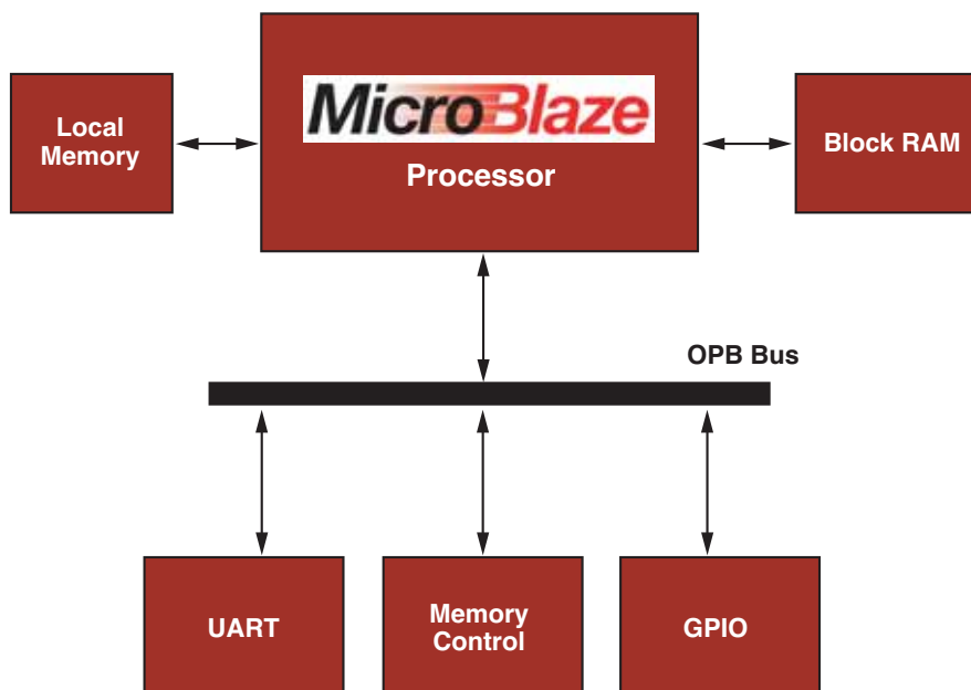
Figure 2 – Typical MicroBlaze configuration
